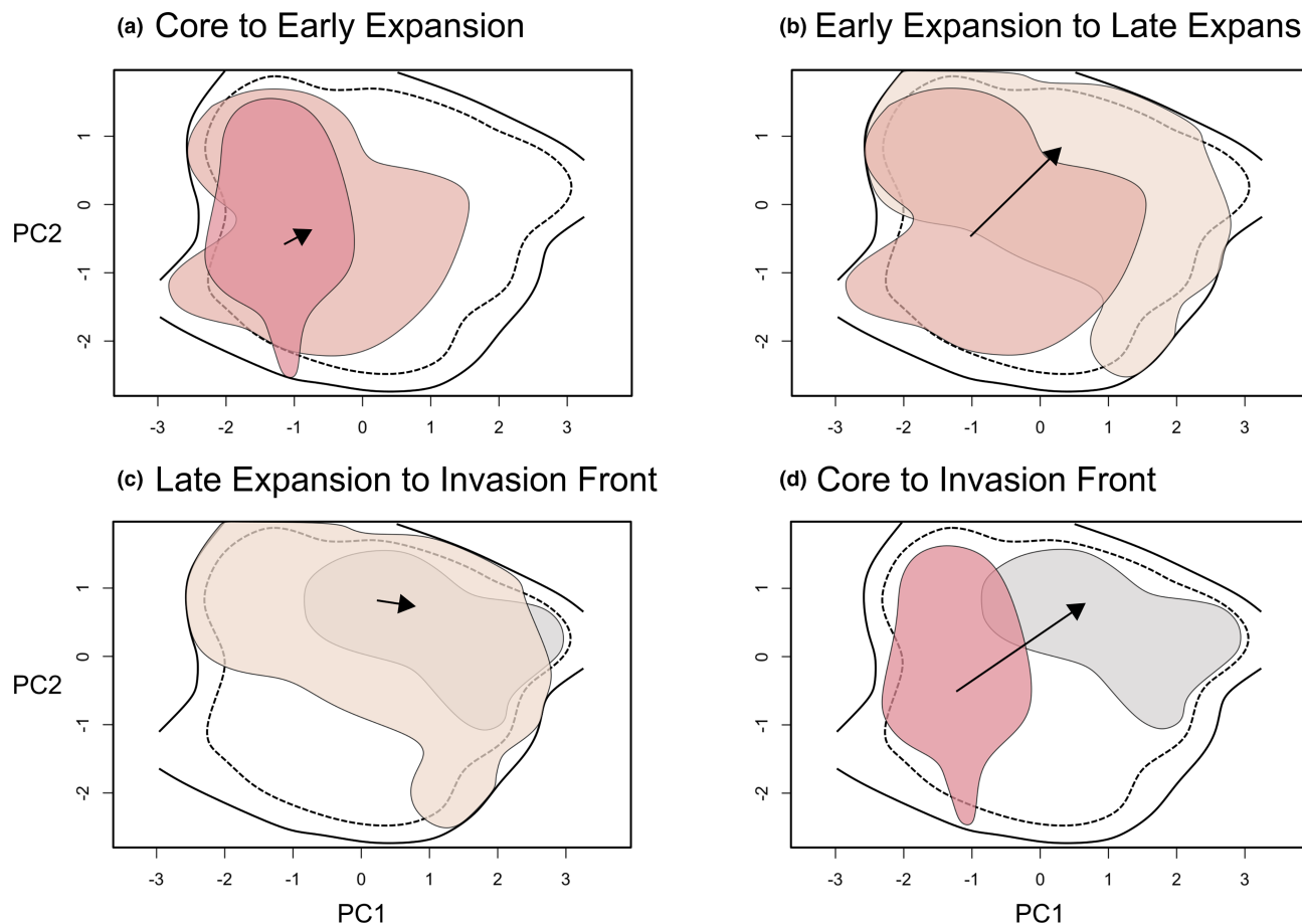
FIGURE 5 Niche overlap during range expansion in climate niche space. The extent of the background environment is outlined in black (solid = total niche space; dashed = 90% of extent). a) Core (dark pink) versus early expansion (light pink), b) Early expansion (light pink) versus late expansion (beige), c) Late expansion (beige) versus invasion front (gray), d) Core (dark pink) versus invasion front (gray). In all panels, the arrow represents the direction of shift in the centroid of niche space.
